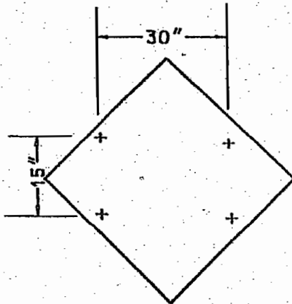
36" DIAMOND
