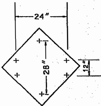
30" DIAMOND
